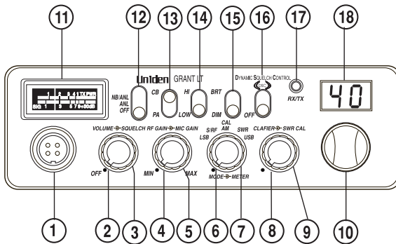
FRONT VIEW - Grant LT BACKLIT PANEL
